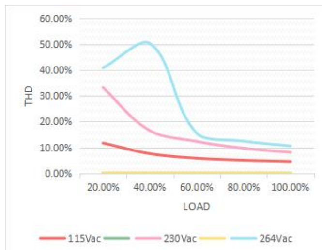
Fig. 4 THD curve
